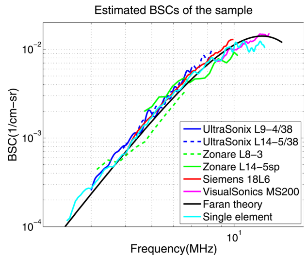
FIG. 2. (Color online) Backscatter coefficients vs. frequency estimates using each of the clinical ultrasound systems. Results are presented for two transducers for both the UltraSonix and the Zonare scanners. Also shown are lab measurements employing single-element transducers. The solid black curve is computed using the theory of Faran.
