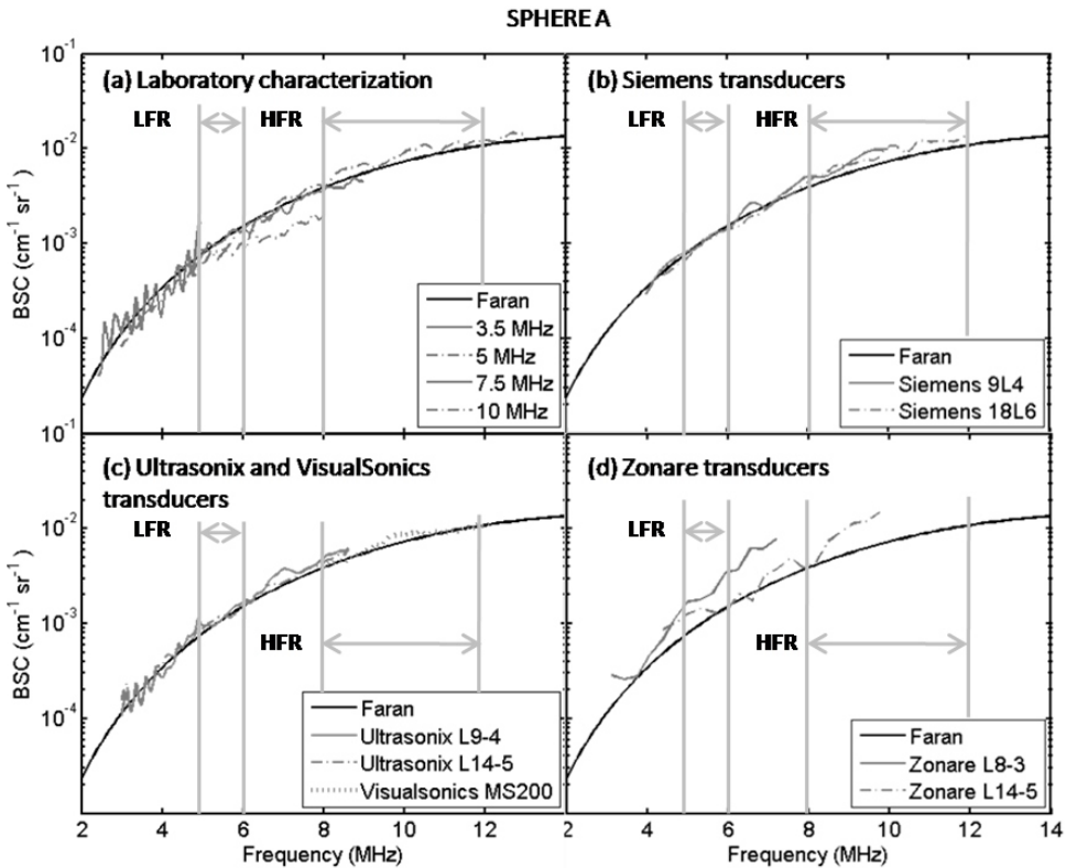
FIG. 4 Experimental estimates and theoretical predictions of the backscatter coefficient of Sphere A as function of frequency. (a) Laboratory characterization using single element transducers, (b) Siemens transducers, (c) Ultrasonix and VisualSonics transducers and (d) Zonare transducers. Vertical bars indicate the low-frequency analysis range (LFR) and the high-frequency range (HFR).
