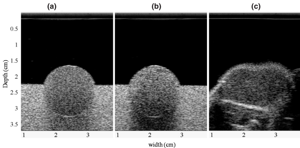
FIG. 3 B-mode images of (a) Sphere A, (b) Sphere B and (c) a spontaneous mammary fibroadenoma in a rat. 15 The three images were acquired with the 9L4 linear array transducer of the Siemens S2000 system under the same scanning parameters.
