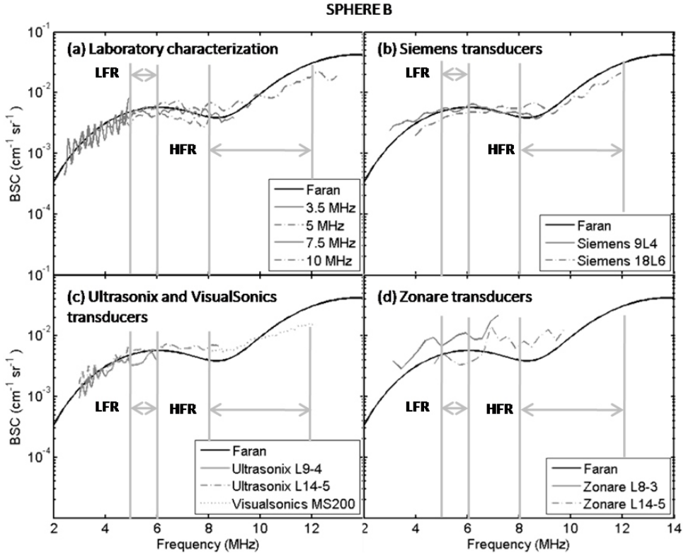
FIG. 5 Experimental estimates and theoretical predictions of the backscatter coefficient of Sphere B as function of frequency. (a) Laboratory characterization using single element transducers, (b) Siemens transducers, (c) Ultrasonix and VisualSonics transducers and (d) Zonare transducers. Vertical bars indicate the low-frequency analysis range (LFR) and the high-frequency range (HFR).
