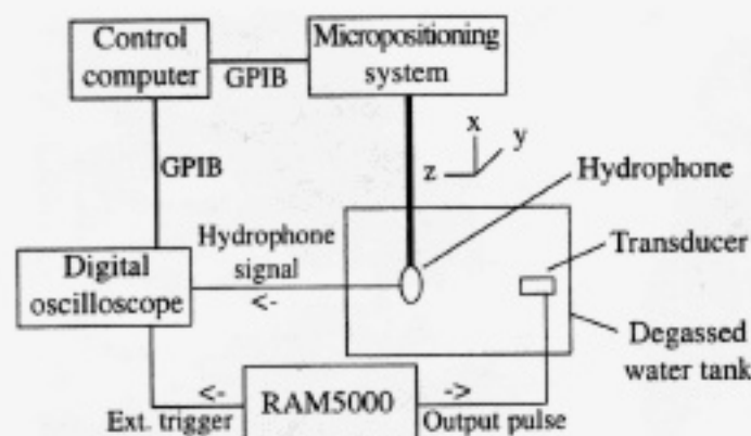
Fig. 1. Block diagram of ultrasound calibration procedure.
